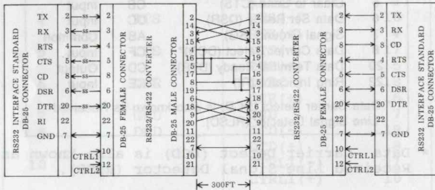
RS232/RS422 CONVERTER BLOCK DIAGRAM (II)
